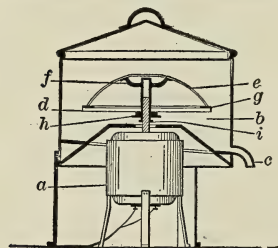
FIG. 197.—Centrifugal Extractor.
